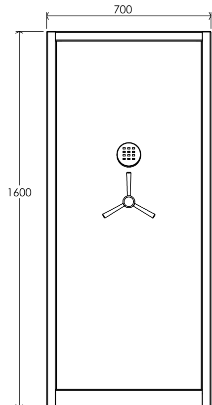
VISTA FRONTAL
